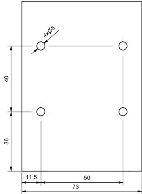
DETAIL A (1 : 1)
