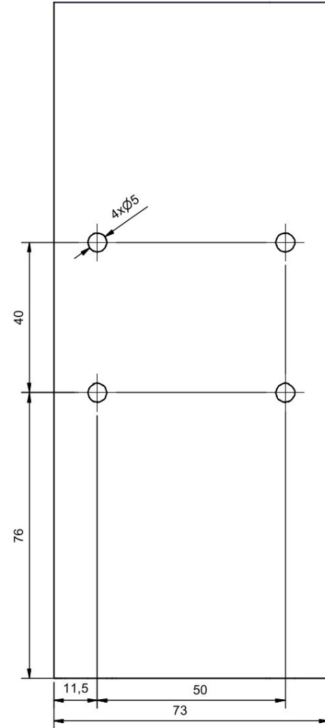
DETAIL B (1 : 1)
